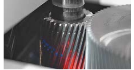
In-process profile and lead measurement with roll testing and laser scanning
